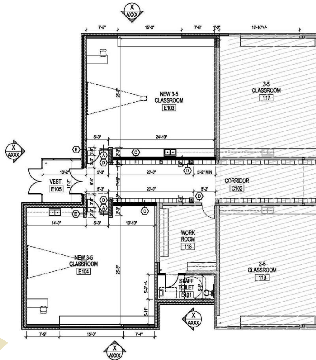
A2 WEST WING FLOOR PLAN A101 1/8" = 1'-0"
