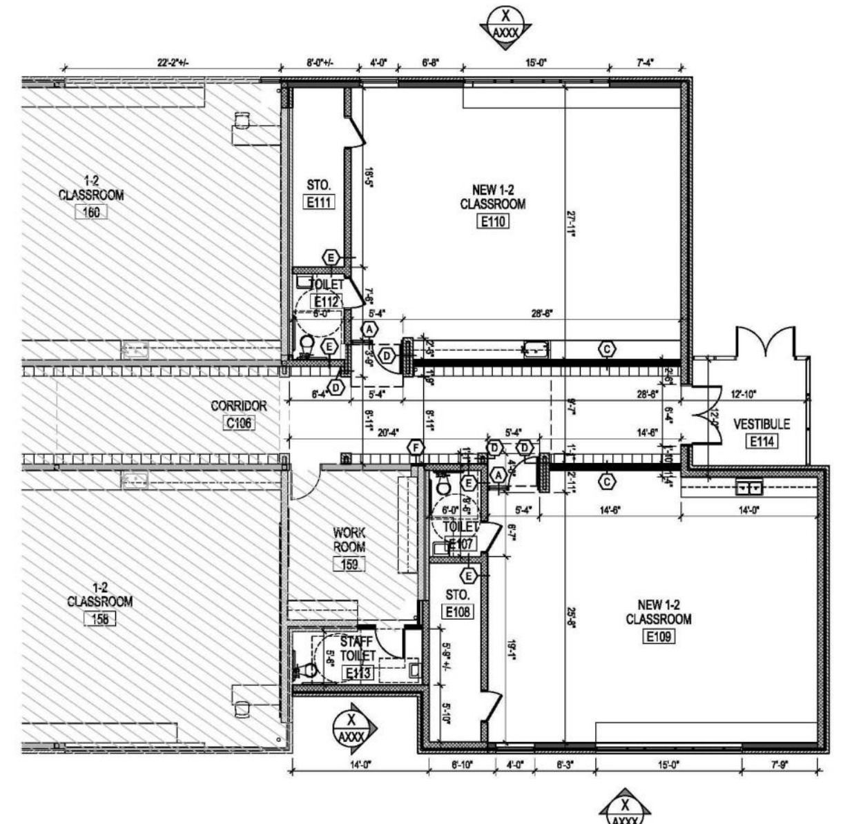
A1 EAST WING FLOOR PLAN A101 1/8" = 1'-0"
